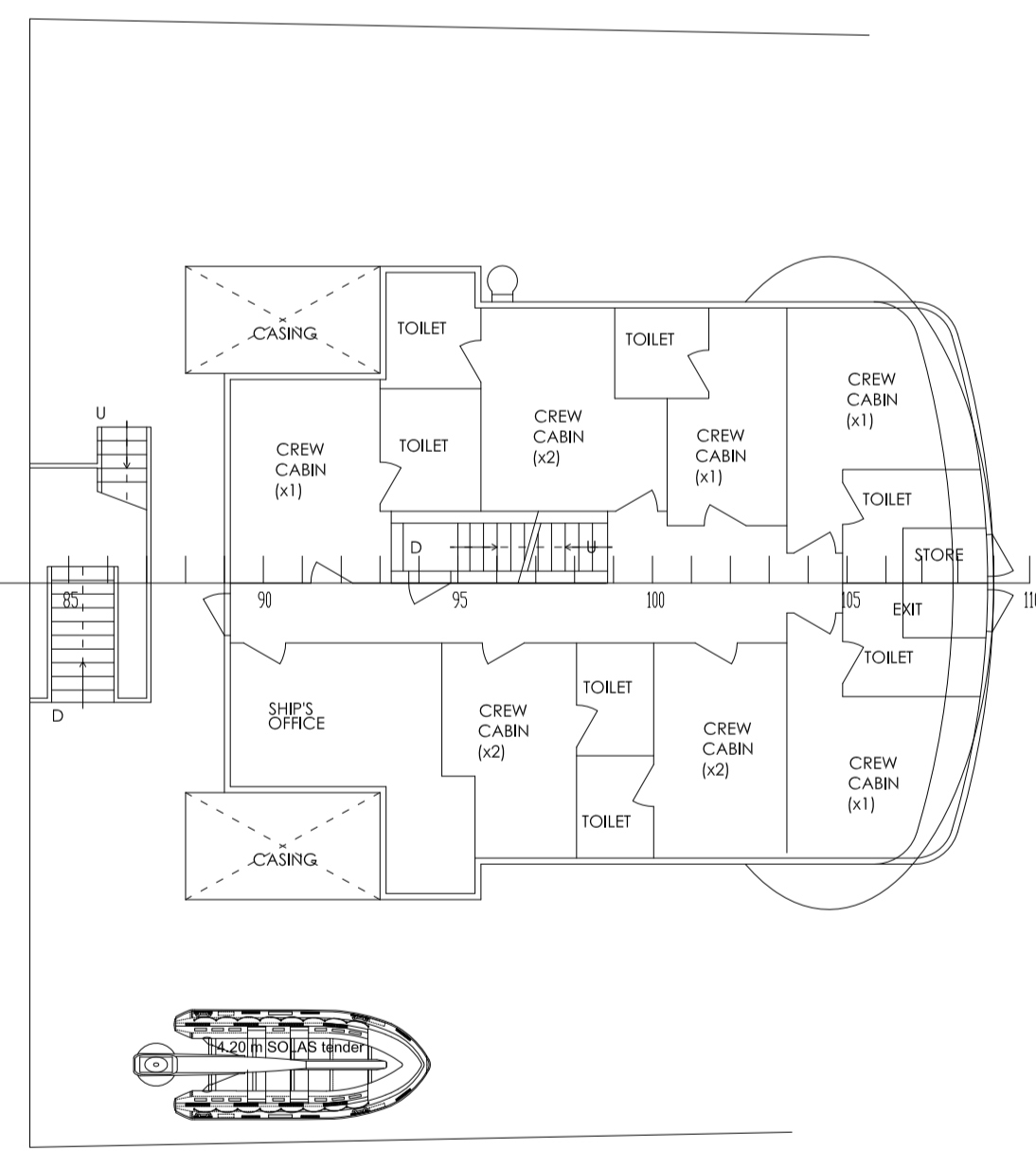
FORECASTLE DECK
