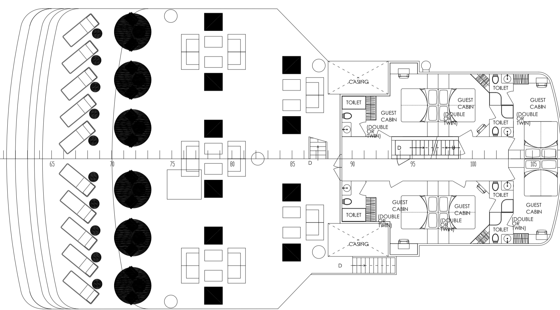
CAPTAIN DECK
