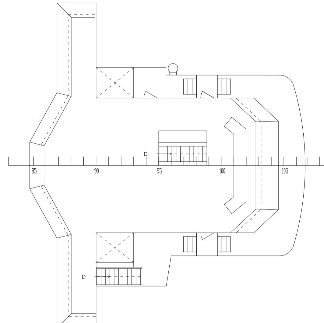
BRIDGE DECK
